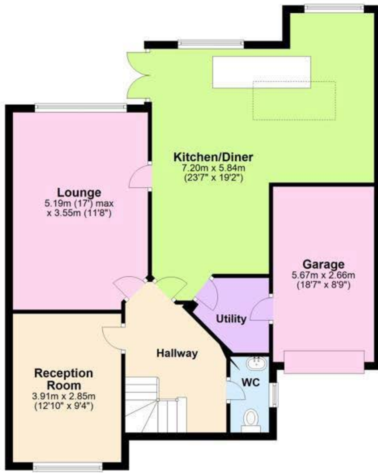
Ground Floor
